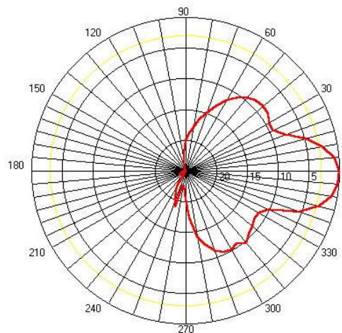
ES24-14 H Plane
