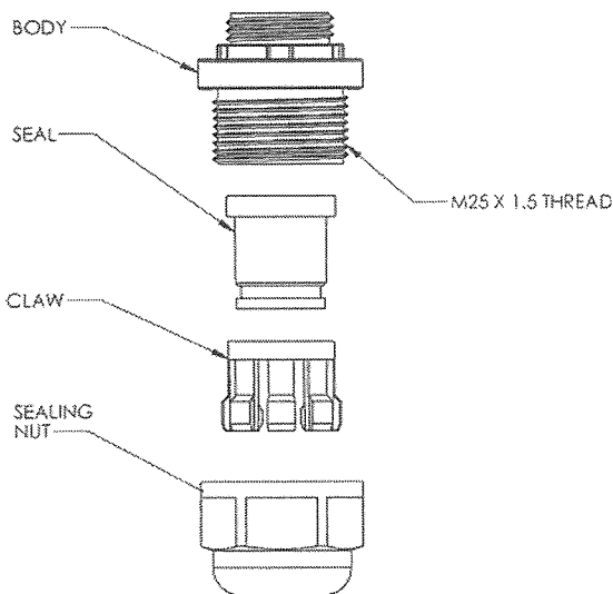
CON-A-2915-01 PARTS
